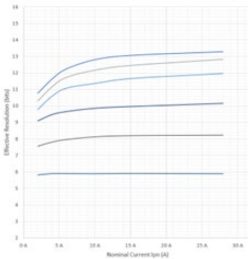
HMSR DA effective resolution vs I_{PN}
