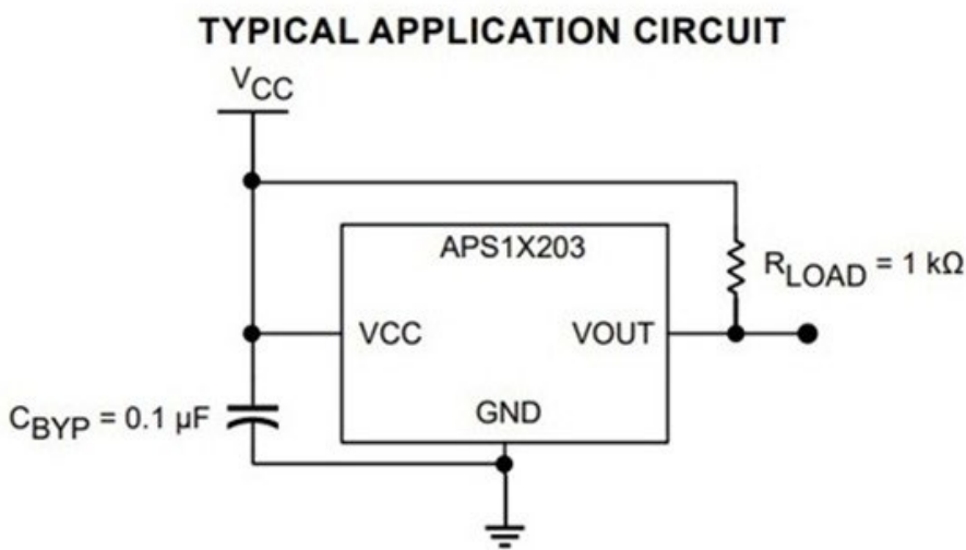
A typical application circuit for Allegro's APS12203. Image source: Allegro Microsystems
