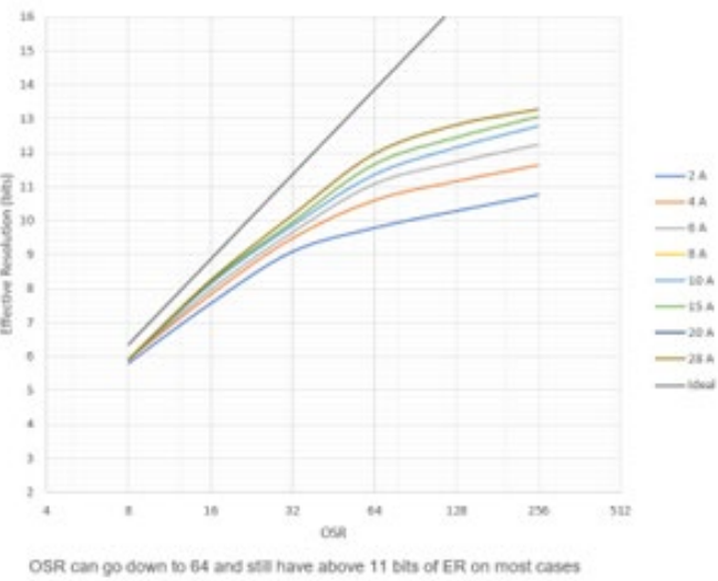
HMSR DA resolution vs OSR (sinc3)
