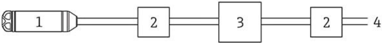
Figure 6: Waterpilot FMX installation block diagram showing the positions of the two surge arresters (2). Image source: Endress+ Hauser
