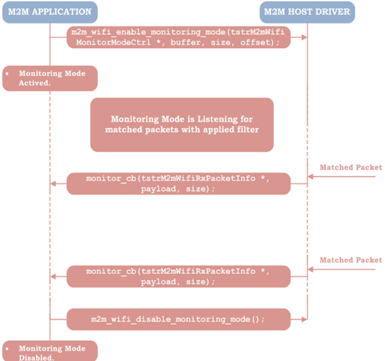
Figure 14-1. Monitoring Mode Sequence Diagram
