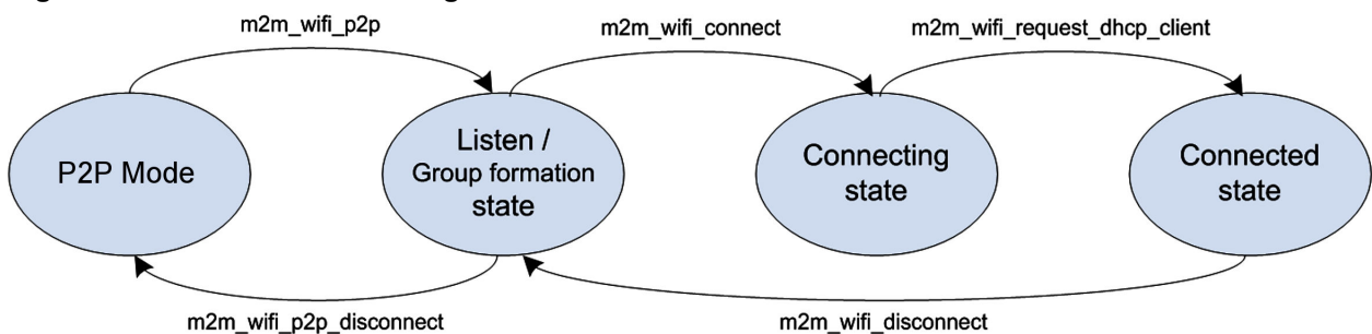
Figure 9-1. P2P Mode State Diagram
