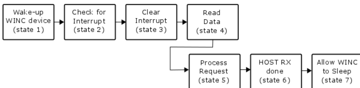
Figure 15-4. HIF Frame Receive from WINC to Host
