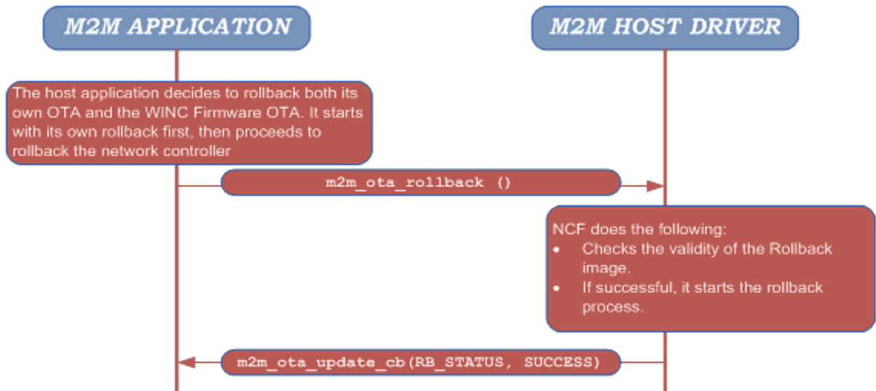
Figure 11-3. OTA Image Rollback Sequence
