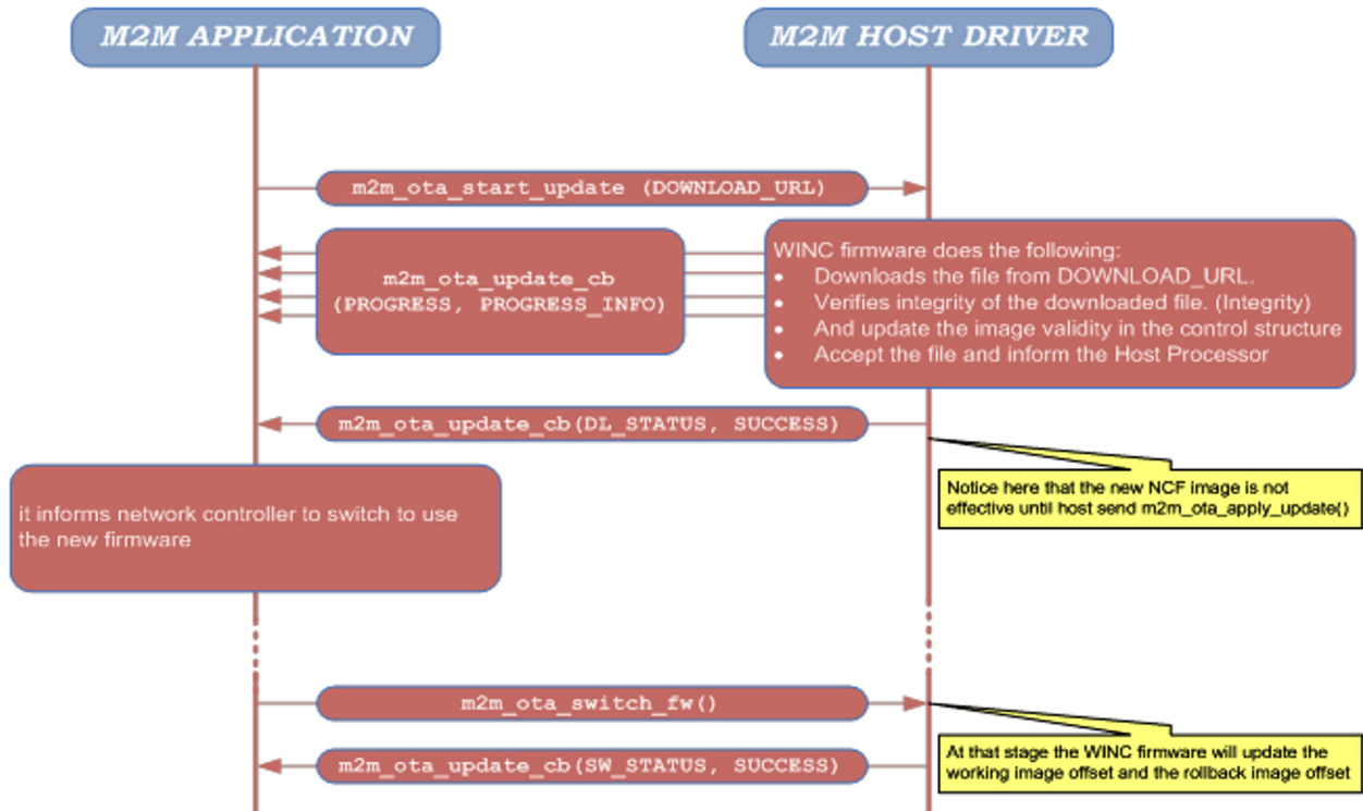
Figure 11-2. OTA Image Download and Install
