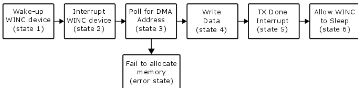
Figure 15-3. HIF Frame Transmit to WINC
