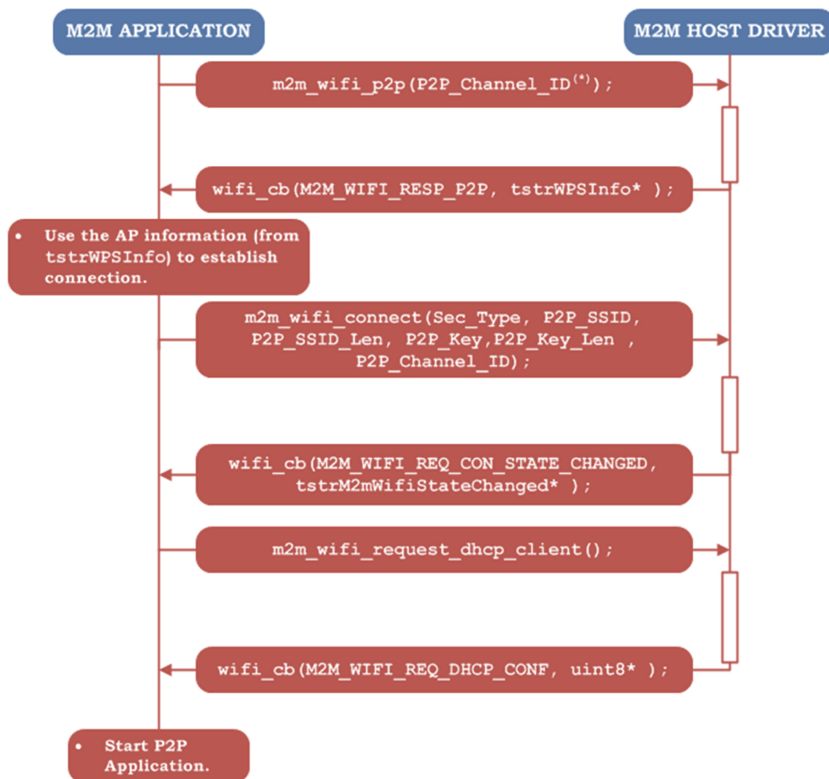
Figure 9-2. P2P Connection Flow
