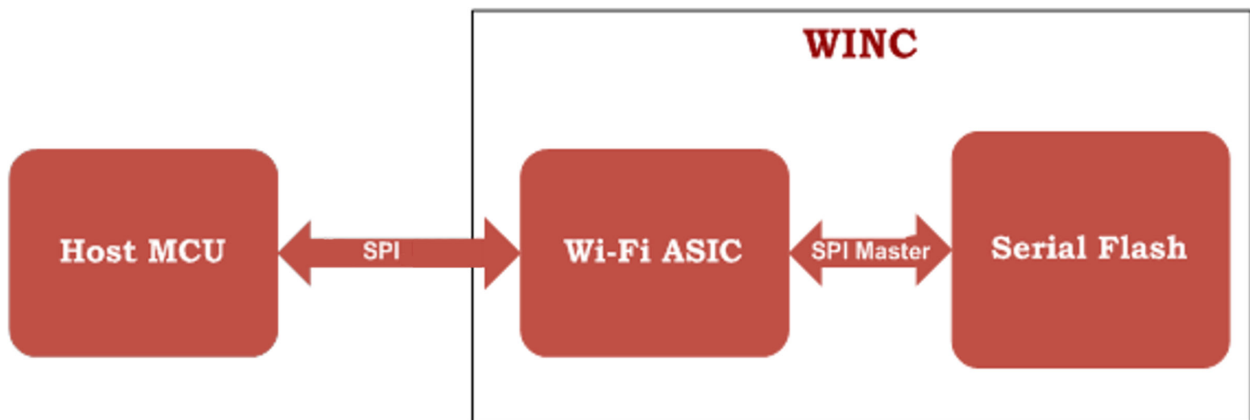
Figure 13-1. System Block Diagram showing SPI Flash Connection
