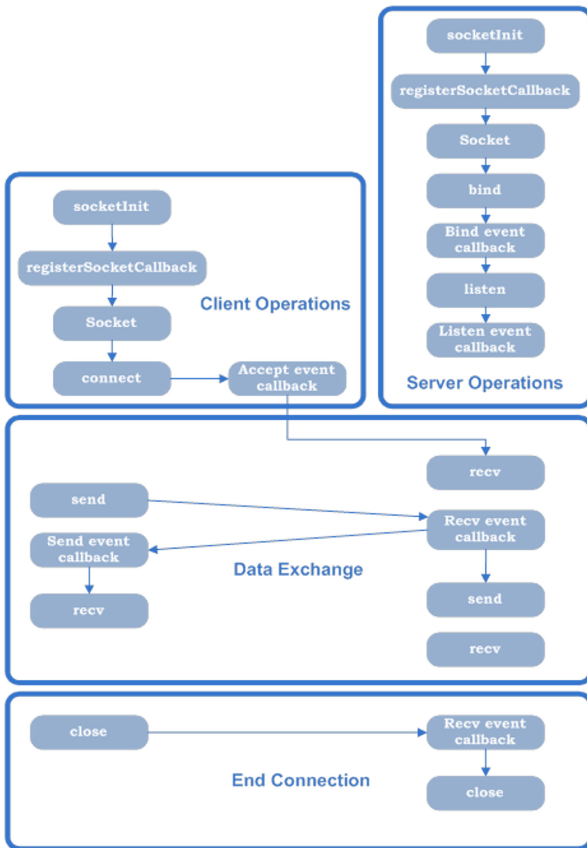
Figure 6-3. Typical Socket Connection Flow
