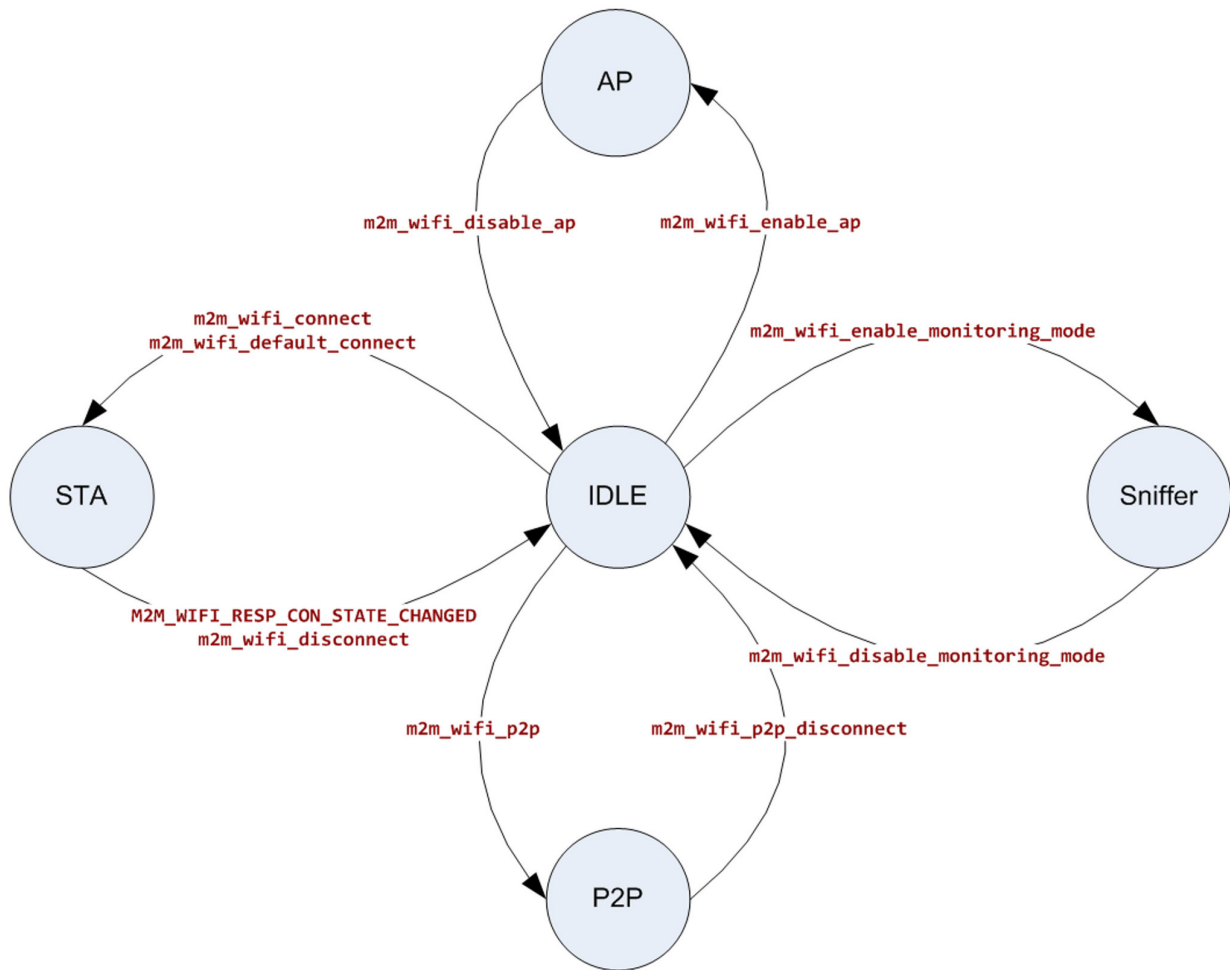
Figure 4-1. WINC Modes of Operation
