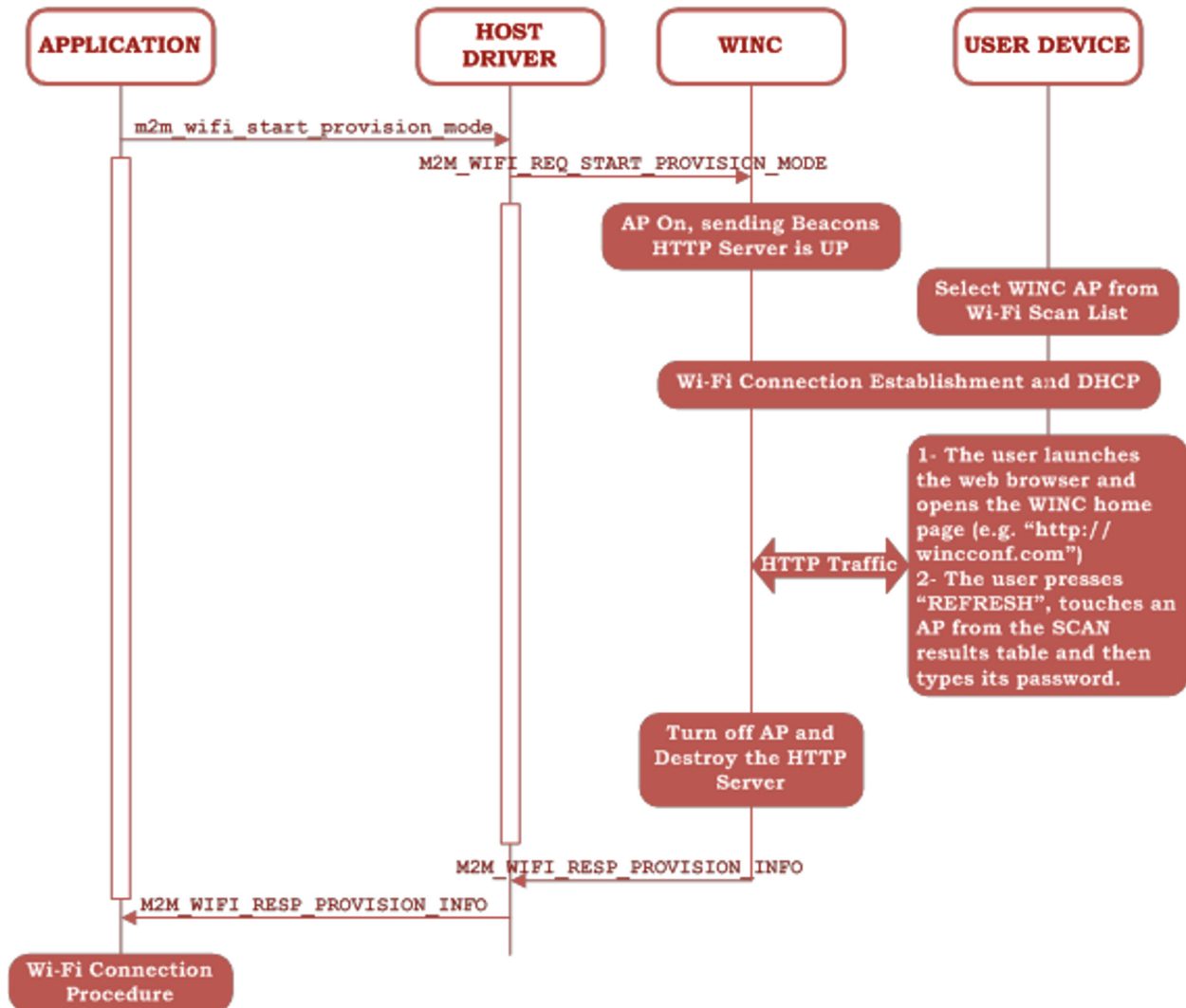
Figure 10-2. HTTP Provisioning Sequence Diagram
