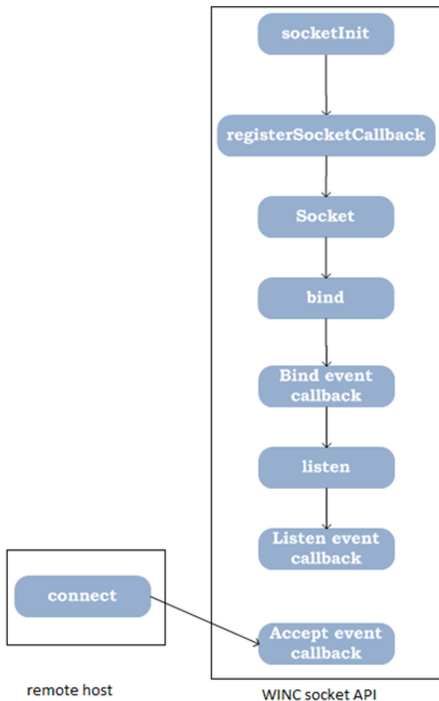
Figure 6-2. TCP Server API Call Sequence
