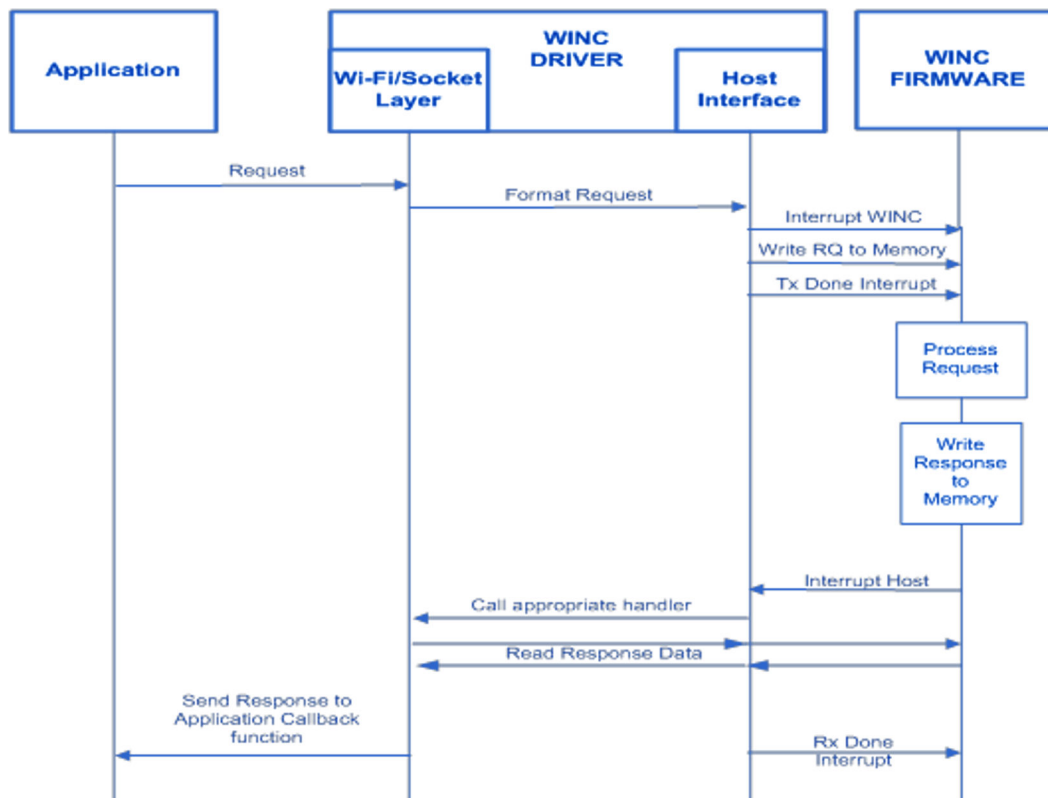
Figure 15-2. The Request/Response Sequence Diagram
