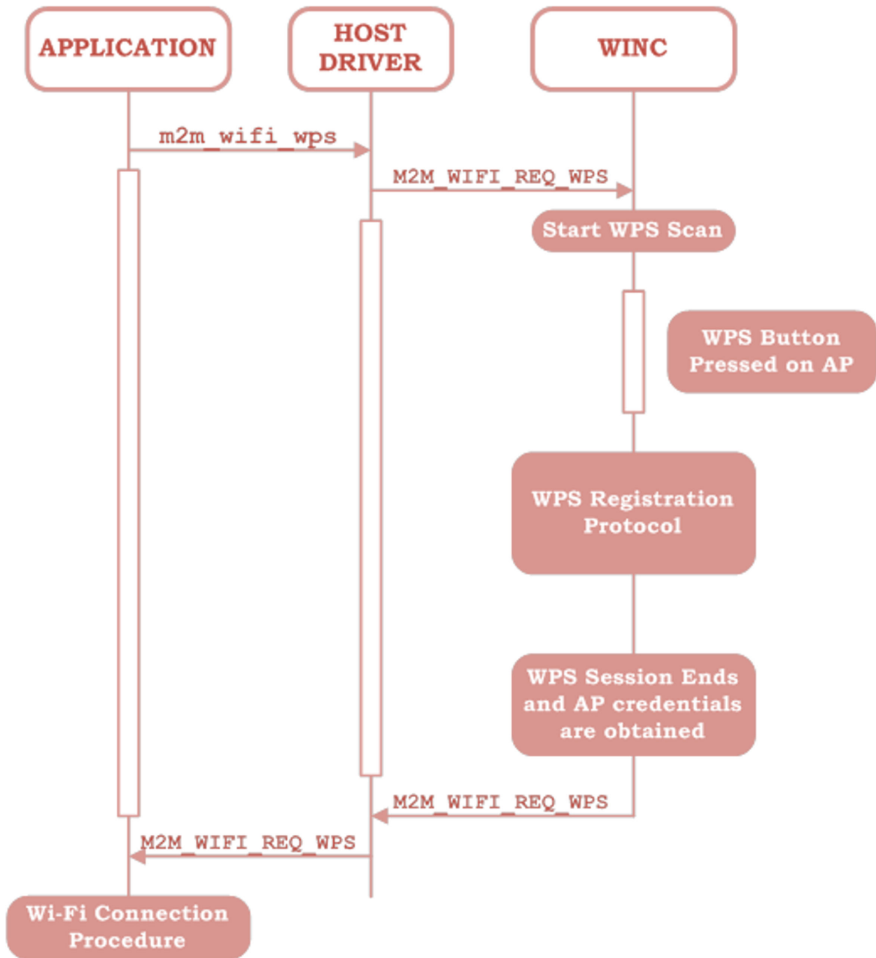
Figure 10-3. WPS Operation for Push Button Trigger
