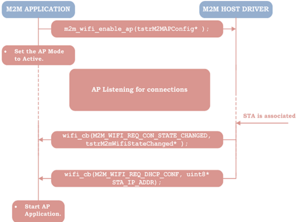
Figure 8-1. WINC AP Mode Establishment
