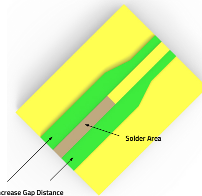
Figure 13 Example of increase the gap distance to improve impedance matching
