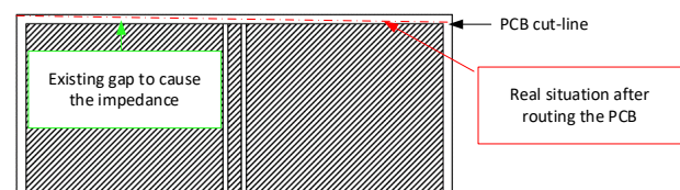
Figure 23 Ground not extended to end of the PCB
