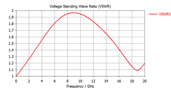
Figure 34 VSWR measurement (Original Design)
