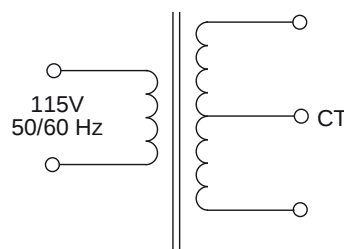
Single Primary
