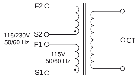
Dual Primary
