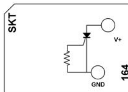
CTJ420E164 One JANTX 2N2323A SCR One 1.1 kΩ Resistor, 1/10 W
