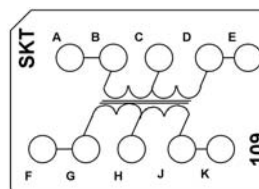
CTJ420E109 One MIL-T-27/172-45 Transformer
