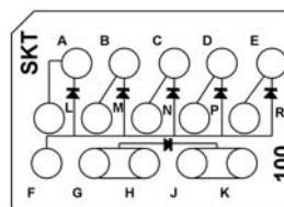
CTJ420E100 Six JANTX 1N5618 Diodes
