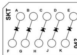
CTJ420E042 Five JANTX 1N5418 Diodes
