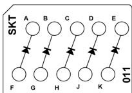
CTJ420E011 Five JANTX 1N5618 Diodes
