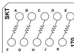
CTJ420E170 Five 249 Ω Resistors, 1/4 W
