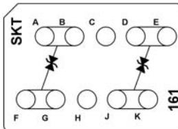
CTJ420E161 Two JANTX 1N6059A Zener Diodes
