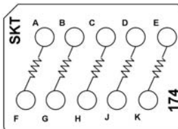
CTJ420E174 Five 100 kΩ Resistors, 1/10 W
