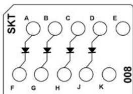
CTJ420E008 Four JANTX 1N3613 Diodes
