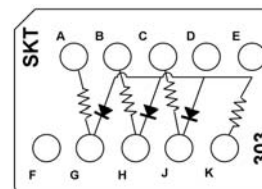
CTJ420E303 One 2.7 kΩ Resistor, 1/4 W One 1.8 kΩ Resistor, 1/4 W One 5.1 kΩ Resistor, 1/4 W One 3.3 kΩ Resistor, 1/4 W Three JANTX 1N5711 Diodes
