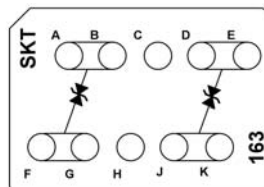
CTJ420E163 Two JANTX 1N6045A Zener Diodes
