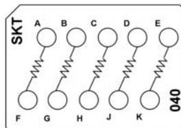
CTJ420E040 Five 49.9 kΩ Resistors, 1/20 W
