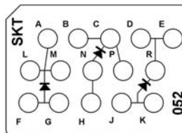
CTJ420E052 Three JANTX 1N5618 Diodes
