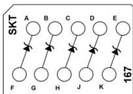
CTJ420E167 Five 1N5351B Zener Diodes
