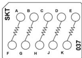
CTJ420E037 Five 23.2 k \Omega Resistors, 1/20 W
