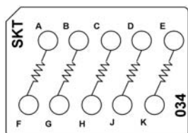
CTJ420E034 Five 150 \Omega Resistors, 1/10 W
