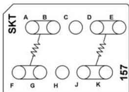
CTJ420E157 Two 120 Ω Resistors, 1/4 W
