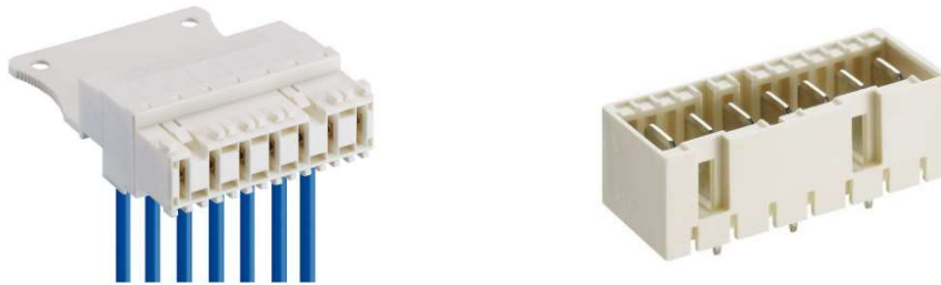
RAST 5 connector for indirect mating, with screw terminal, lift clamp and protection against misplacing.
