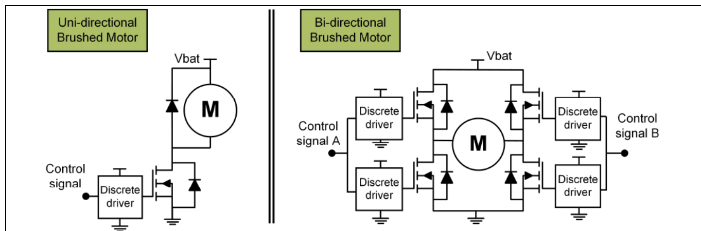
Figure 5 Brushed DC common drive circuits for uni-directional motors and bi-directional motors
