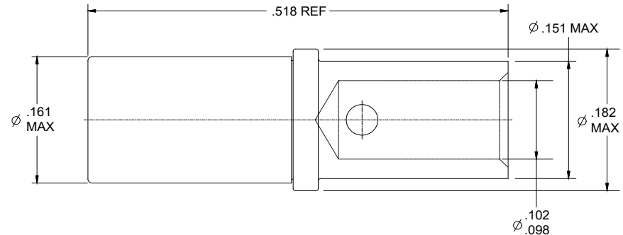
Socket - 980-0008-877
