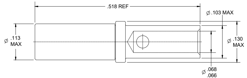
Socket - 980-0008-876
