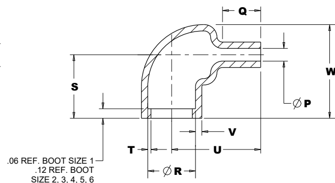
RIGHT ANGLE BOOT (AS RECOVERED)
