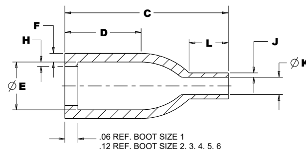
STRAIGHT BOOT (AS RECOVERED)
