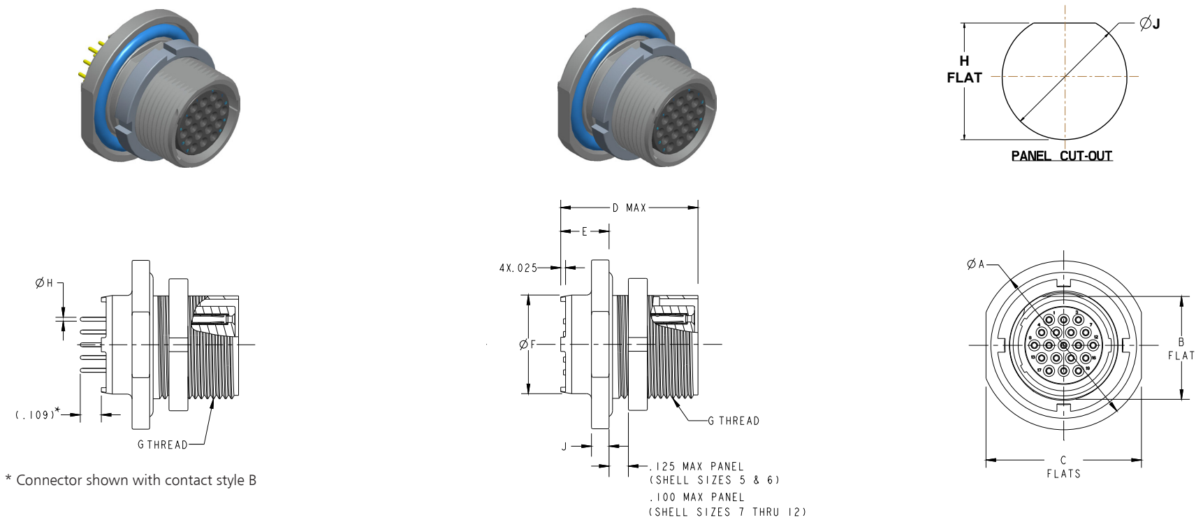
MKJ0 Jam Nut Receptacle - Rear Panel Mount PCB PC Tail
