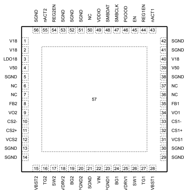
56-LEAD (8mm x 8mm) PLASTIC QFN EXPOSED PAD (PIN 57) IS SGND. MUST BE SOLDERED TO PCB.
