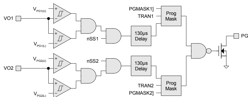
Powergood logic
