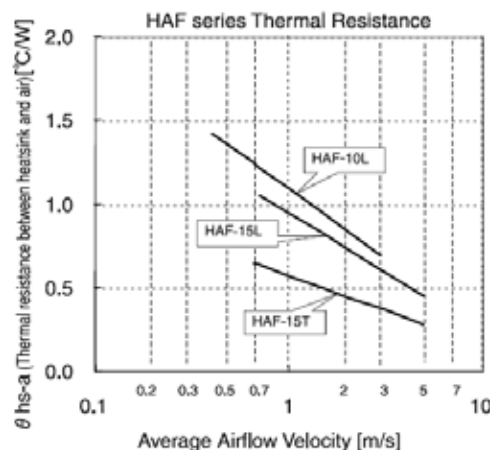
Fig. 4: Thermal resistance of heatsinks with airflow
