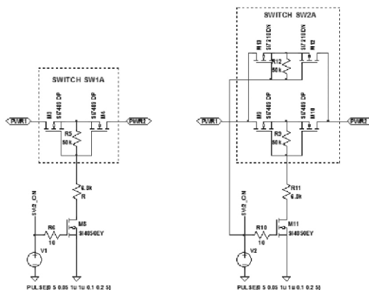
Fig. 8 - SWITCH SW A - Bi-directional switch for switching voltages PWR1, PWR2 > 4 \text{ V} SWITCH SW B - Bi-directional switch for switching voltages PWR1, PWR2 > 0 \text{ V}
