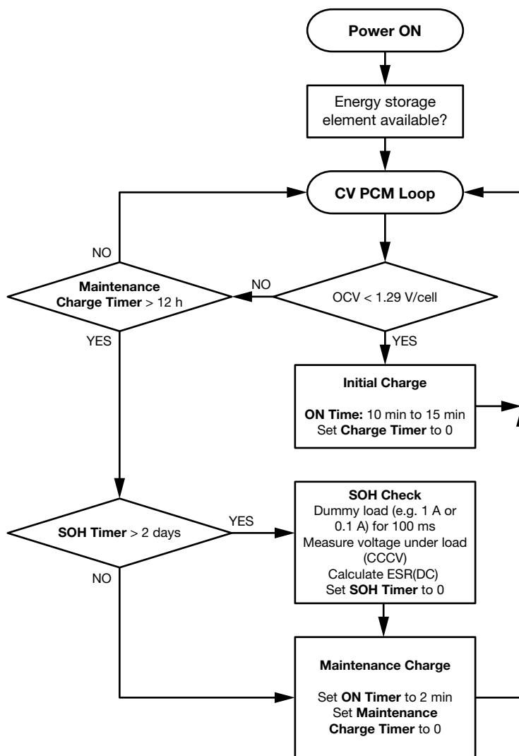
Fig. 1 - Flowchart for operation of a backup system with pulsed charging method
