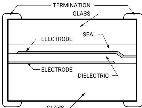
ACCU-P CAPACITOR
