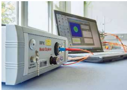
Prevention of attenuations and reflections through end-face testing in fiber-optic cables
