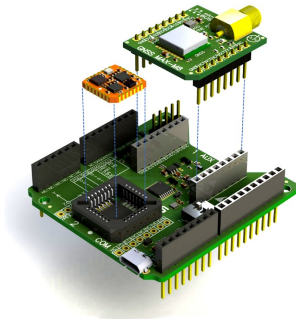
Figure 1: Exploded view of the MTi 1-series Shield board
