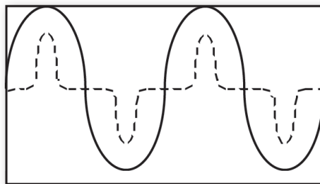
Figure 3. Voltage waveform is sinusoidal, current waveform is non-sinusoidal but in-phase; PF < 1.
