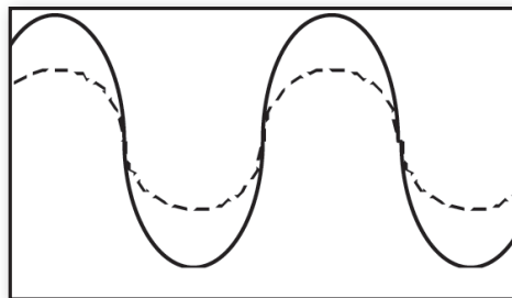
Figure 2. Voltage and Current waveforms are sinusoidal and in-phase; PF=1.
