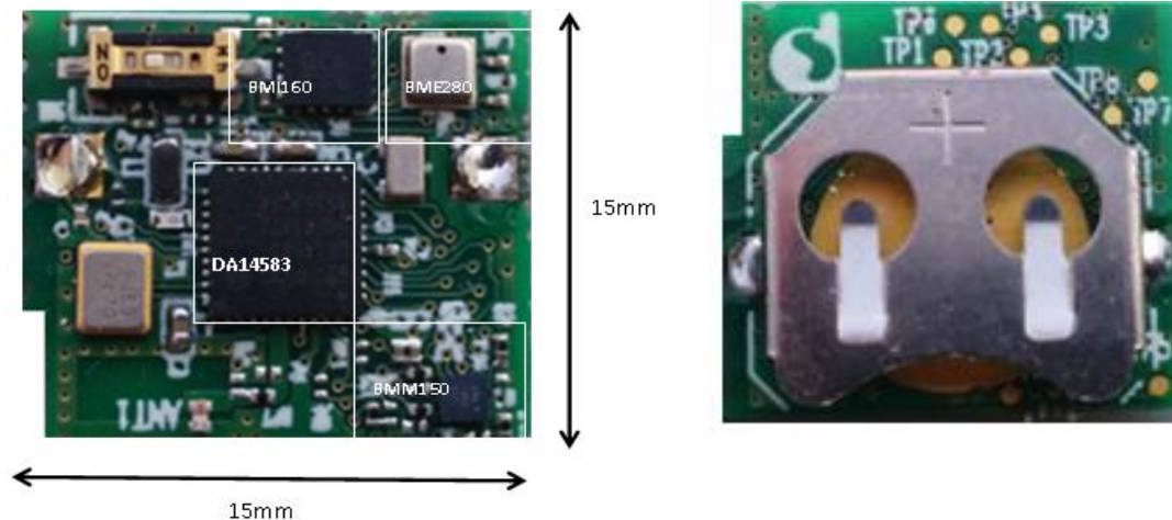
Figure 3: The actual wearable PCBA, top (left) and bottom view (right)
