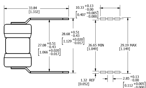
TLS-LSA Dimensions are mm (in)
