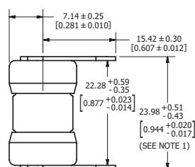
TLS-LSE Dimensions are mm (in)
