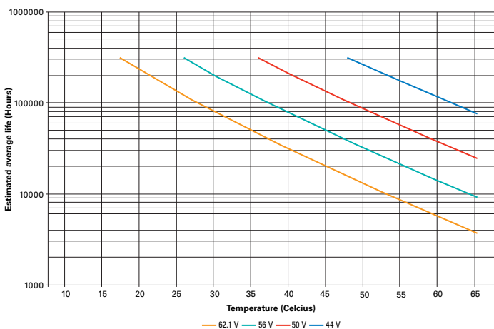
Figure 2. XLM-62 life plot at 62.1 V, 56 V, 50 V, and 44 V.
