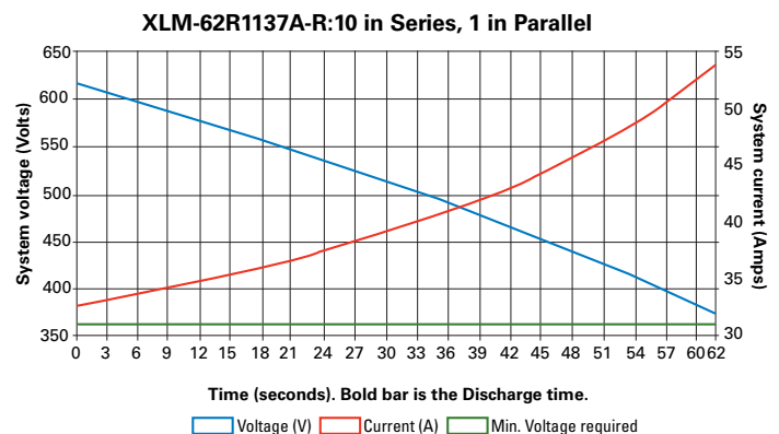
Figure 4. XLM-62R1137A-R calculator output using Figure 5 inputs.
