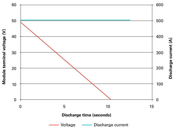
Figure 1b. Example voltage and current discharge curves for 500 A discharge from one module with 56 V float voltage.
