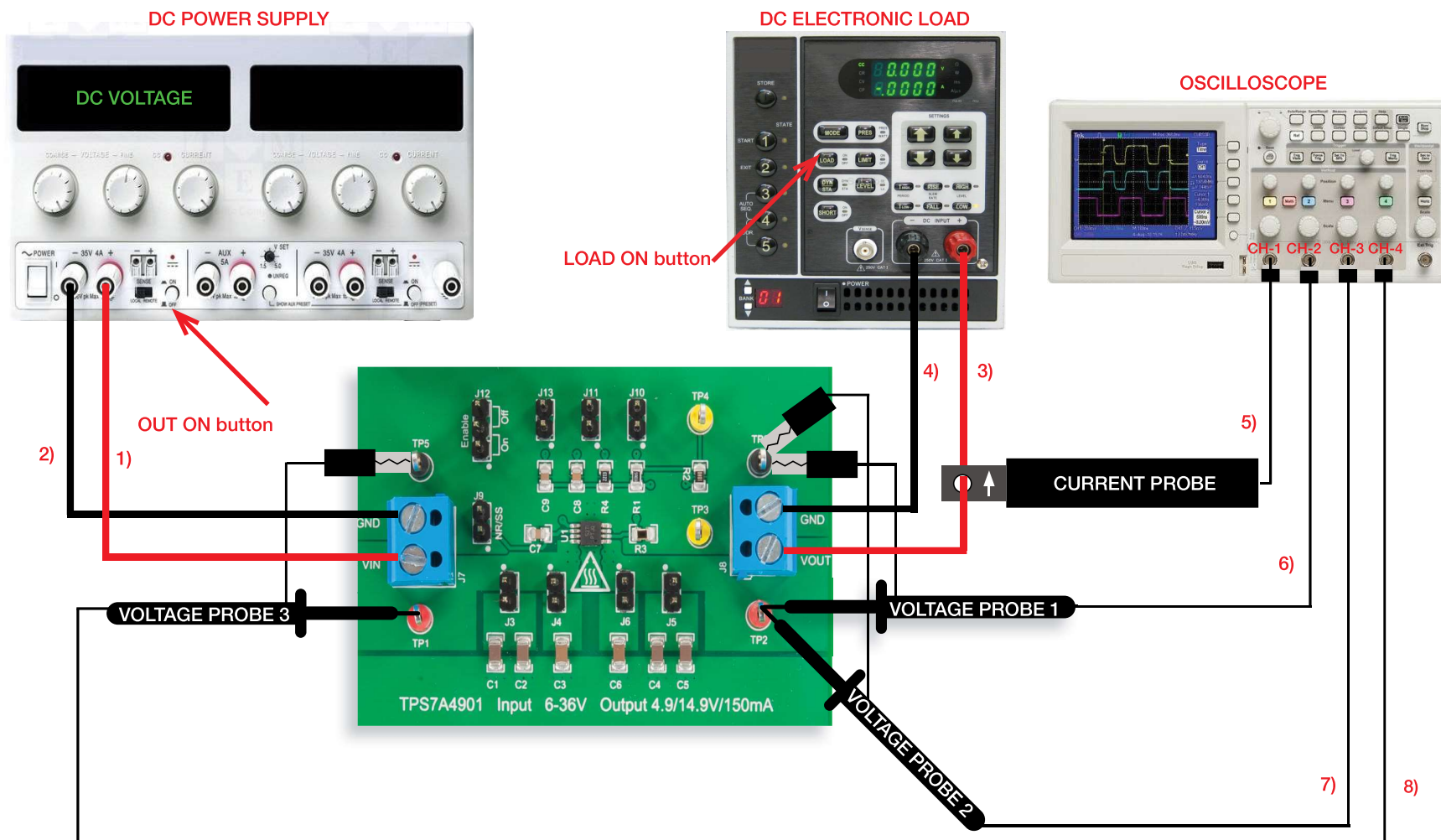
Figure 5. Experiment set-up.
