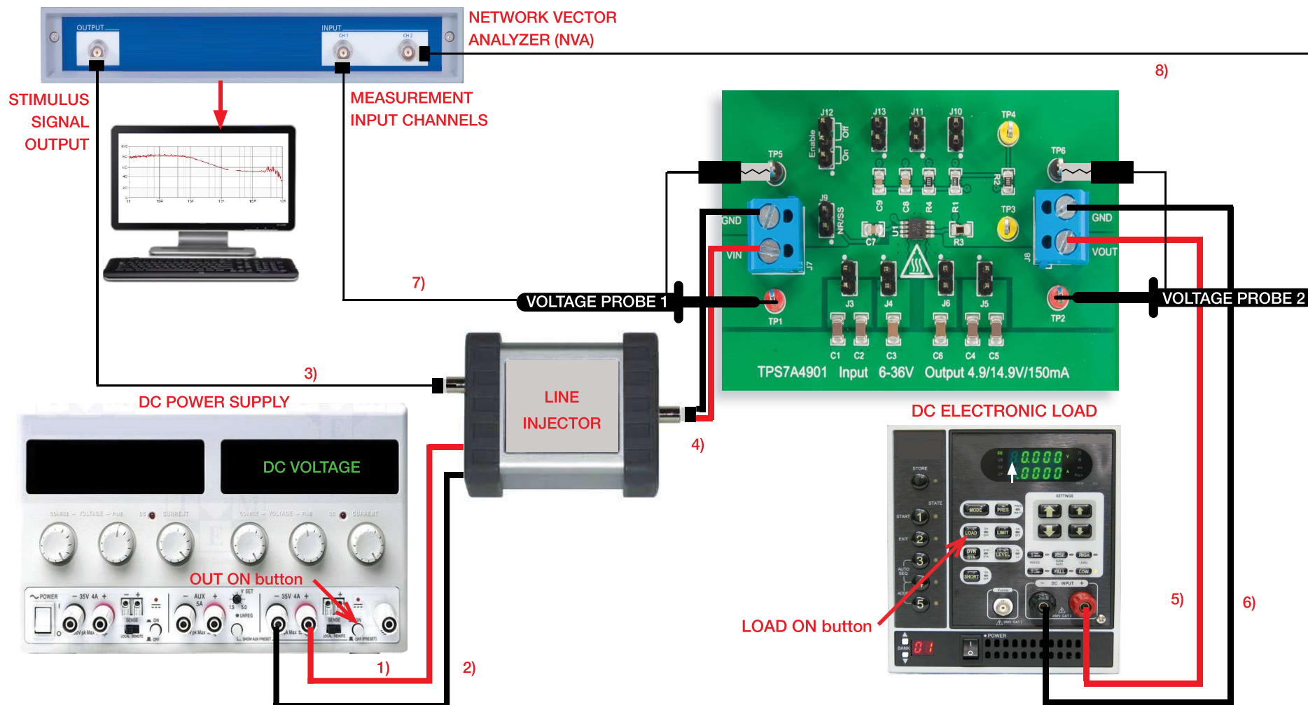
Figure 5. Experiment set-up.
