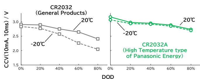
Figure 7. Pulse-Discharge Characteristics at Room Temperature and Low Temperatures
