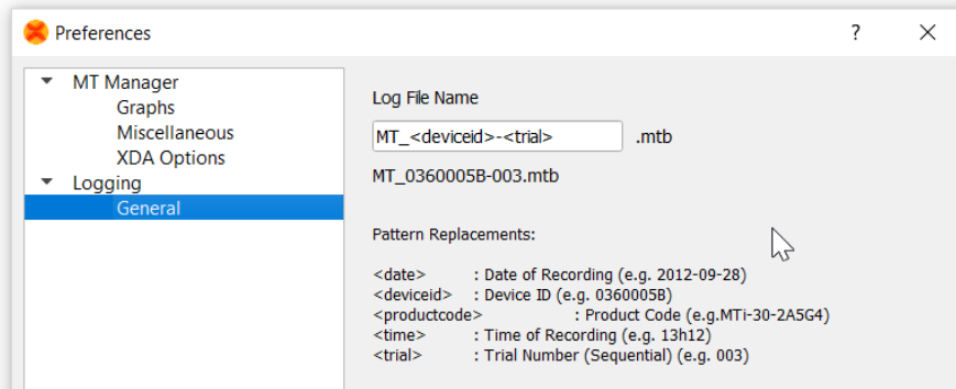
Figure 78: The logging name can be changed in the Preferences window. Use <time> and/or <trial> to ensure unique file names
