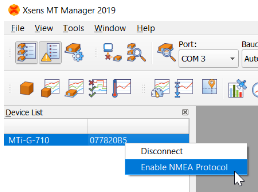
Figure 56: Right-click on the MTi in the Device List and choose "Enable NMEA protocol" to parse data into binary packets in MT Manager. Configure String report mode first to see this option
