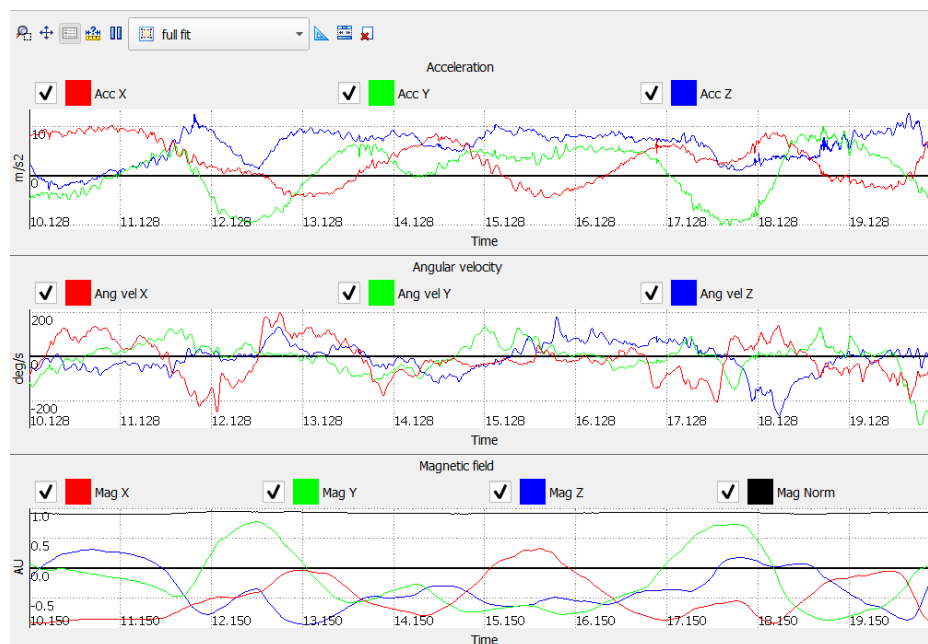
Figure 22: The Inertial data view for acceleration, angular velocity and magnetic field
