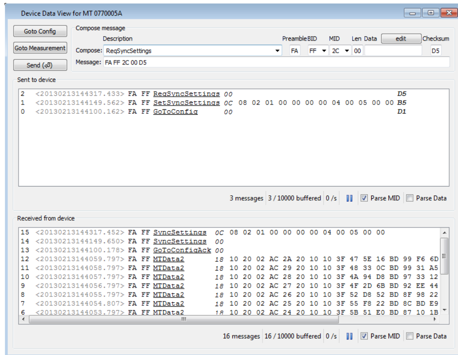
Figure 76: An example showing how to request settings from the MTi device.
