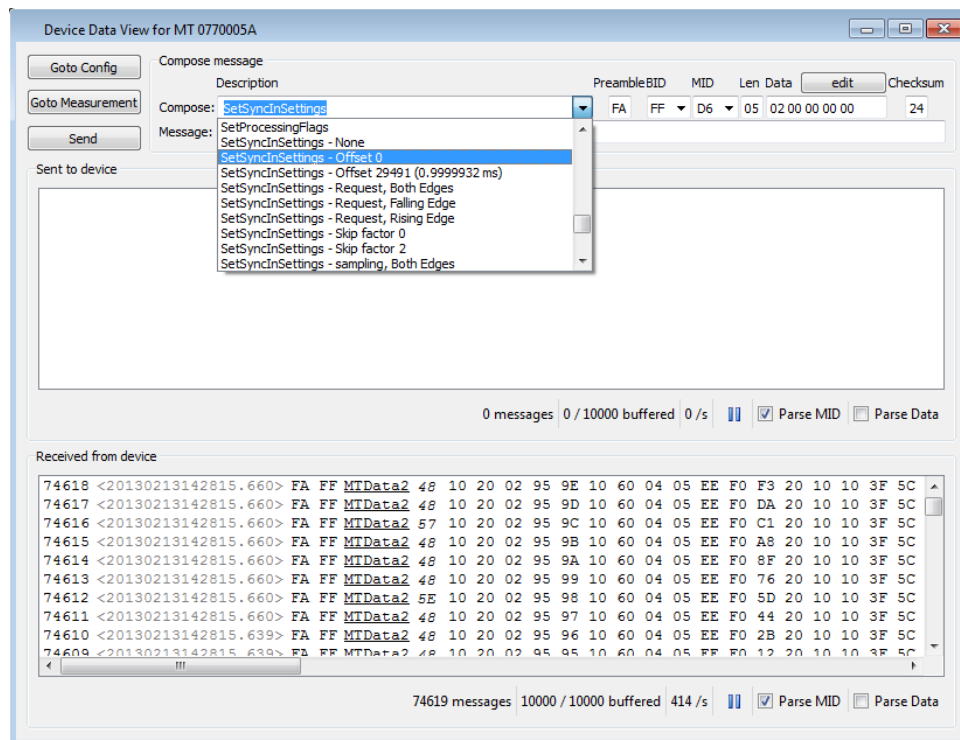
Figure 72: Composing a message in the Device Data Viewer can be done by selecting a message from the "Compose" menu
