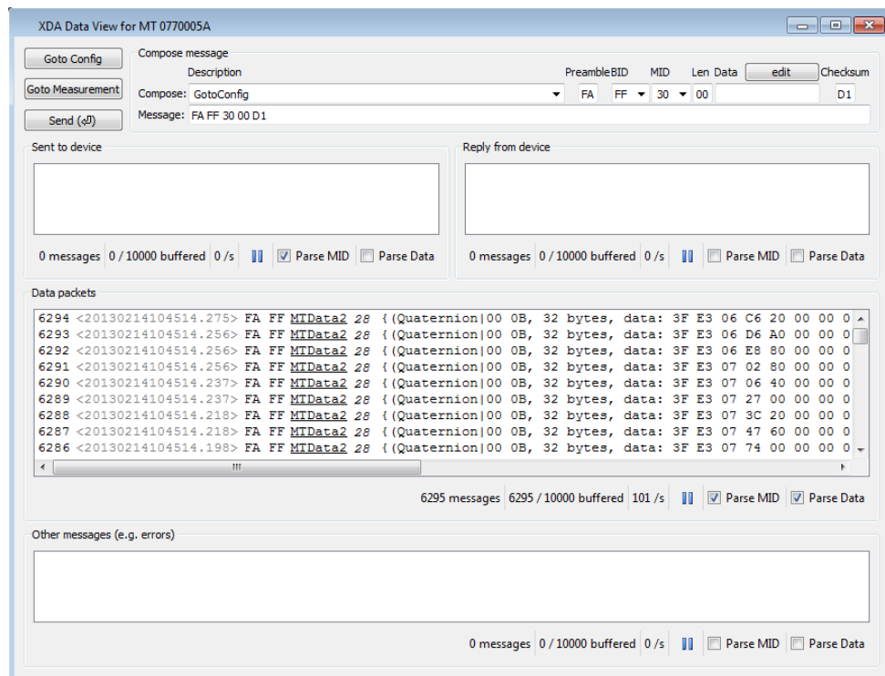
Figure 77: The XDA message terminal has an extra field with respect to the Device Data Viewer, showing the data received from the Xsens Device API (XDA)
