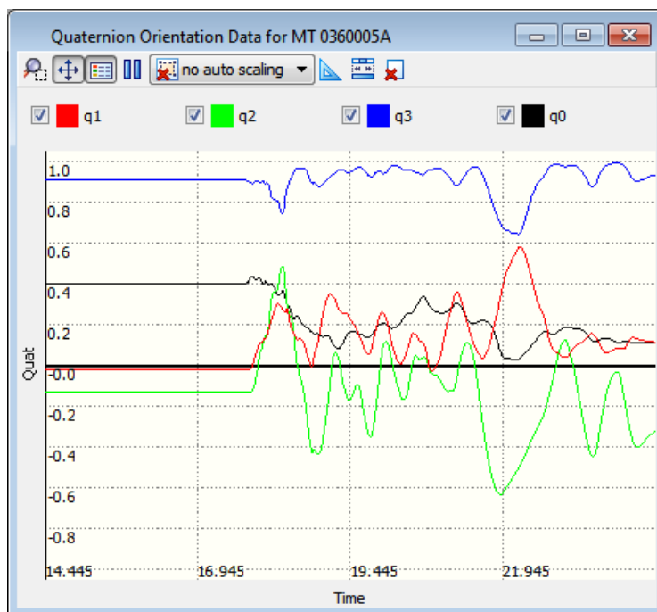
Figure 30: The quaternion graph shows the 4 components in one graph
