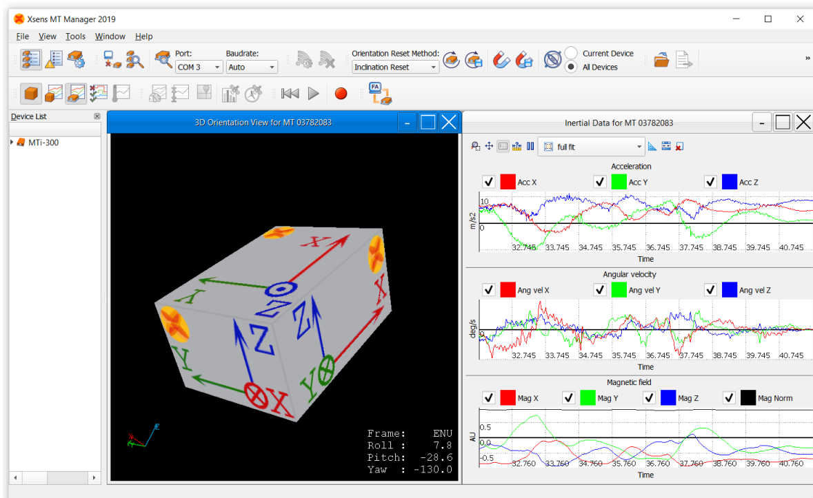
Figure 11: A typical view of MT Manager
