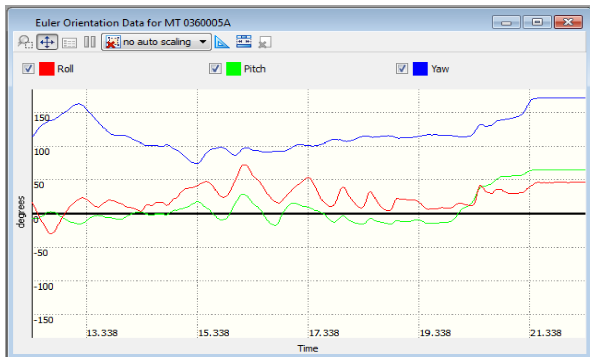
Figure 29: The orientation graph shows the orientation of the MTi over a period of 10 seconds
