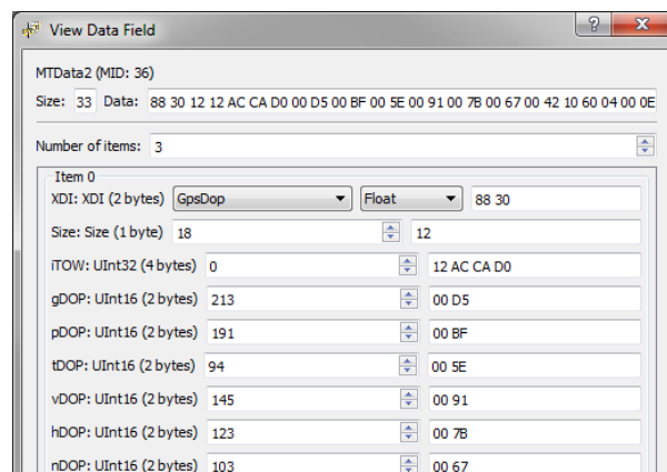
Figure 70: Double-clicking the data field will show the items and values in the data packet
