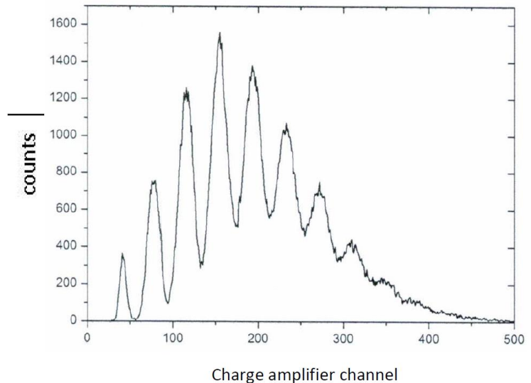
Figure 31. Typical photoelectron spectrum recorded with SiPM coupled to charge amplifier
