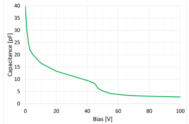
Figure 14. Typical capacitance for APD-800
