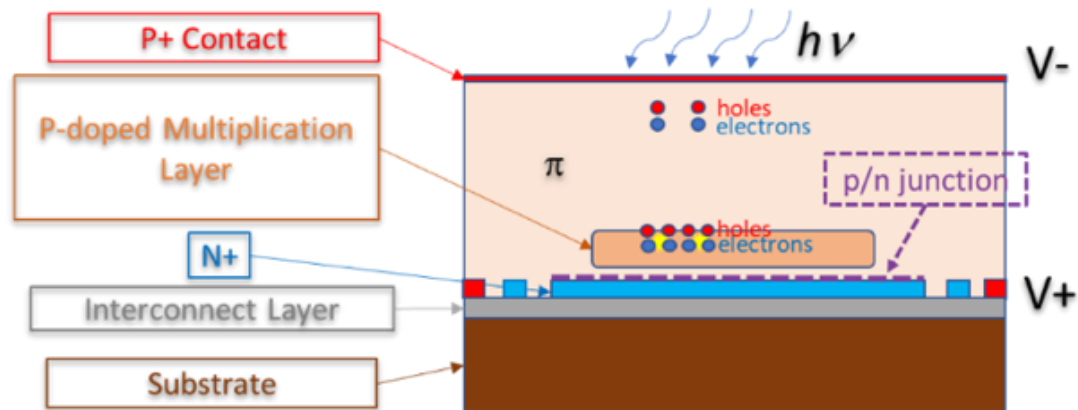
Figure 15. Schematics of a typical backside-illuminated APD
