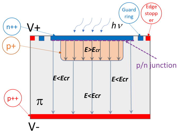
Figure 3. Reach-Through APD Structures with a p+ multiplication layer (p-well) highlighted with light purple color
