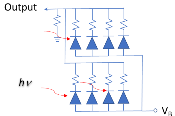
Figure 26. Electrical block-schematics of SiPM
