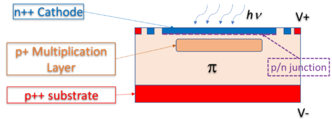
Figure 9. APD structure with buried multiplication layer
