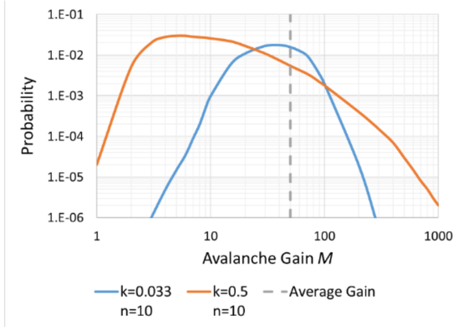
Figure 2. Probability for n injected electrons/holes to result in M*n avalanche electrons/holes
