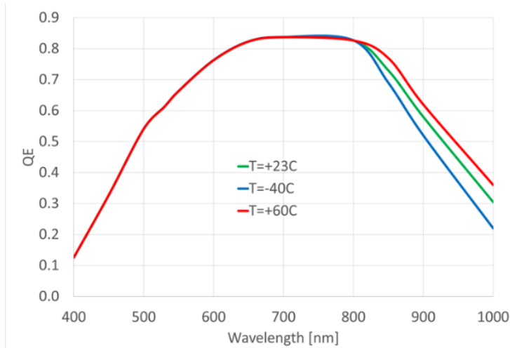
Figure 19. APD-800 QE with temperature for M=1 .
