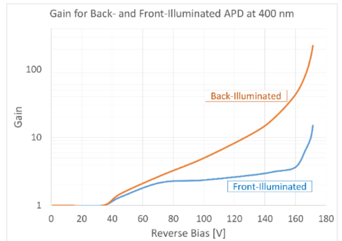
Figure 17. Gain of sample back-illuminated and front-illuminated APDs at 400nm
