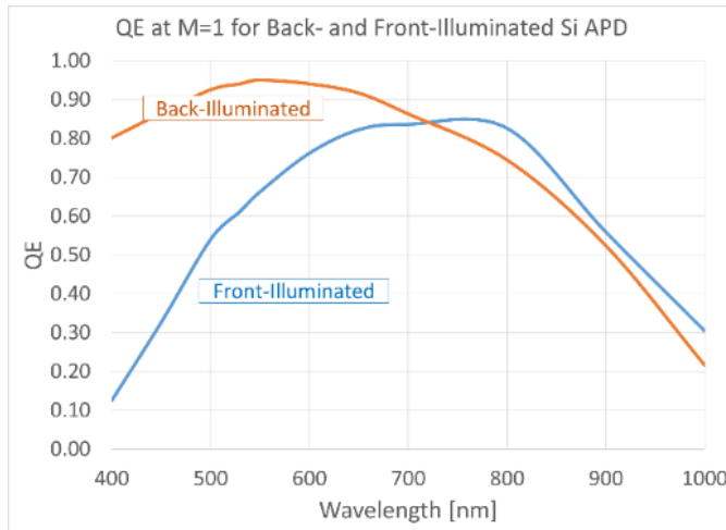
Figure 16. Quantum efficiency of a sample back-illuminated APD
