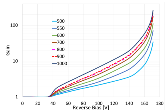
Figure 13. Typical gain of APDE-800 for various wavelengths
