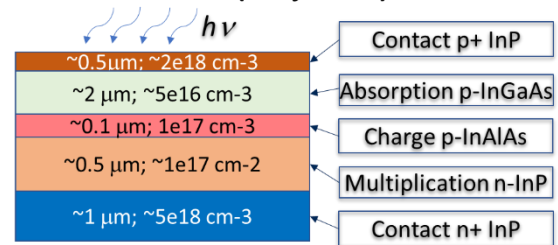
Figure 6. Ge-Si APDs with Separate Absorption and Charge Multiplication regions
