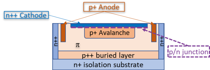
Figure 21. Schematic example of a Geiger-mode APD
