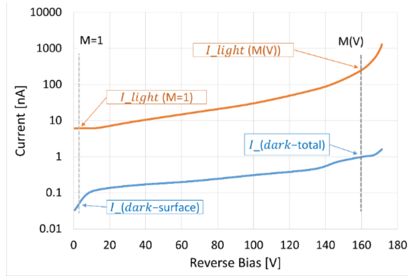
Figure 18. Definitions of the dark and photocurrent for noise calculation
