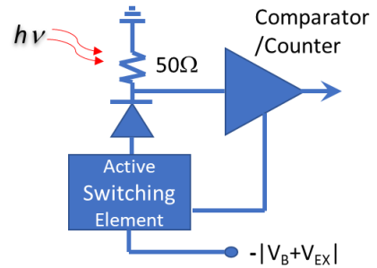
Figure 24. Example of avalanche active quenching
