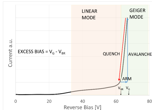
Figure 22. Schematic diagram showing operation of Geiger-mode APDs
