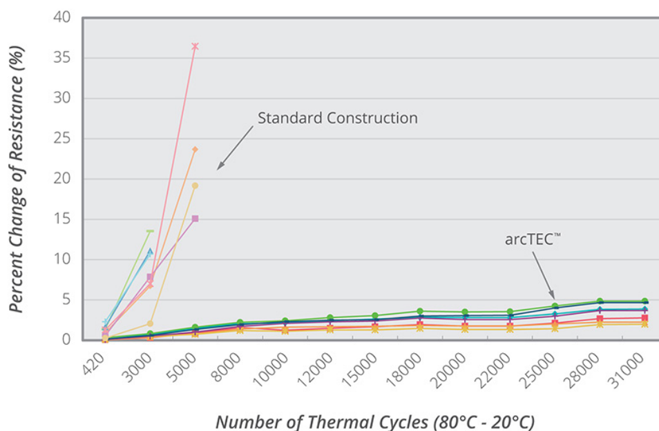
Reliability Test arcTEC™ vs. Standard Construction
