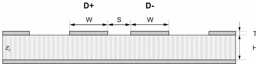
Figure 8: USB differential pair, controlled impedance parameters
