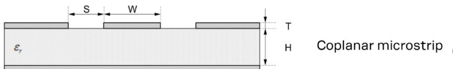
Figure 33: Coplanar microstrip dimension specification
