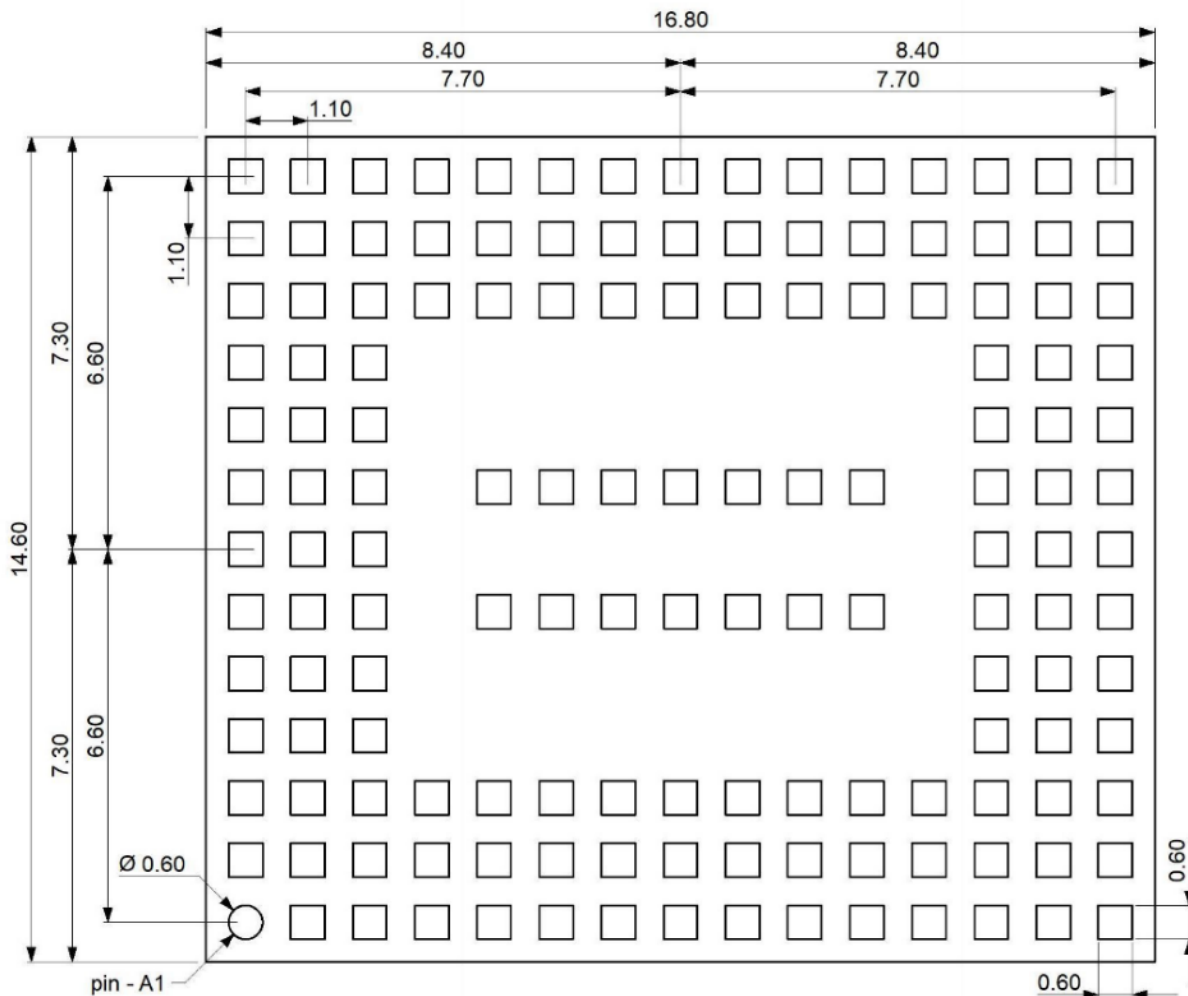
Figure 9: IRIS-W101 recommended PCB footprint (top view)
