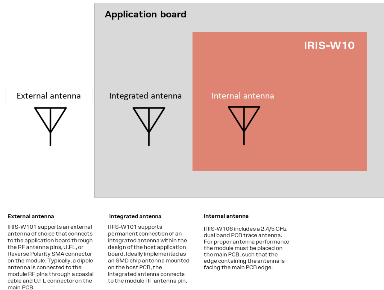
Figure 3: Antenna options
