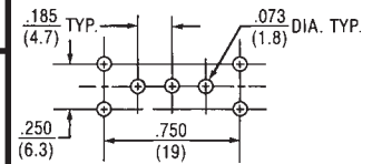
1 Pole P.C. Mounting
