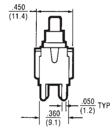
DP
