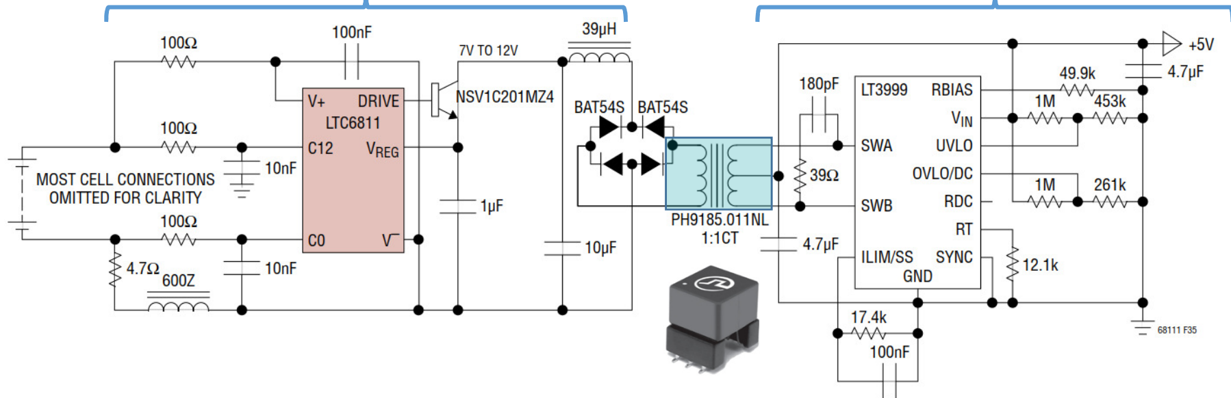
Multicell battery stack monitor
