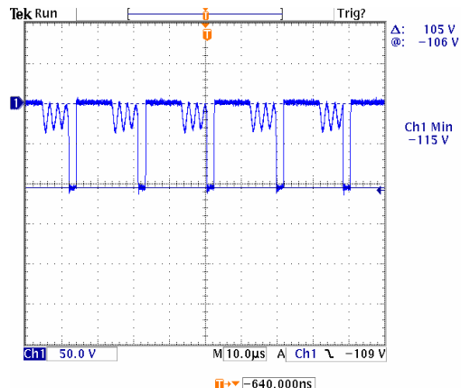
Shut down VAK wave form @ 264Vac/50Hz, full load
