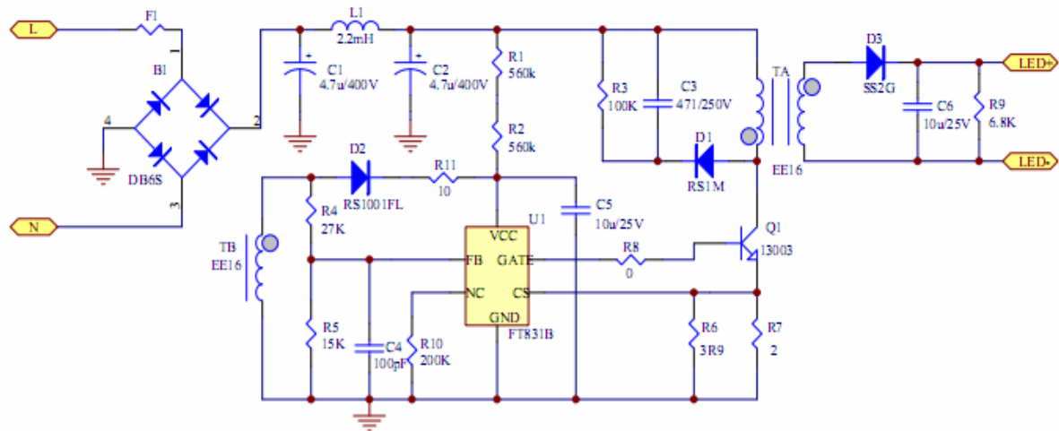
Figure 1: Schematic
