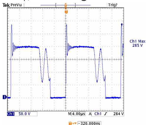
Start up, Vds wave form @ 90Vac/50Hz
