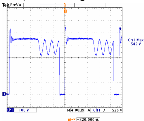
Start up, Vds wave form @ 264 Vac/50Hz
