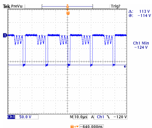
Start up VAK wave form @ 264Vac/50Hz, full load
